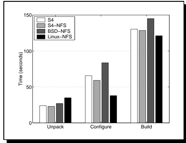
Figure 4: SSH-build Benchmark
