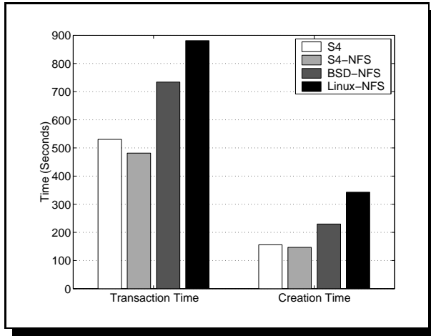
Figure 3: PostMark Benchmark
